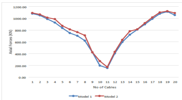
[Graph 1: Comparison between Axial Cable Forces]
