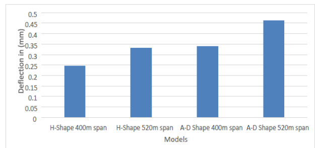
[Graph 9: Variation in Displacement between H-Type and A-D Type Bridge]
