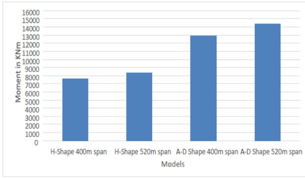
[Graph 11: Variation in Bending Moment between H-Type and A-D Type Bridge]
