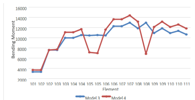
[Graph 6: Variation between Bending Moment]
