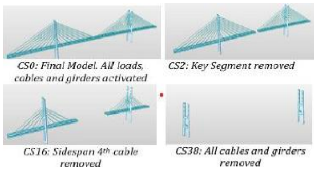
[Fig.5: Backward Analysis Sequence]
