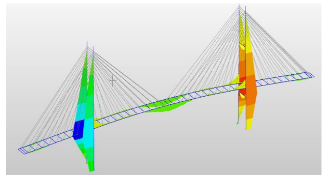
[Fig.3: Bending Moment Prior Unknown-Load Factor Optimization]
