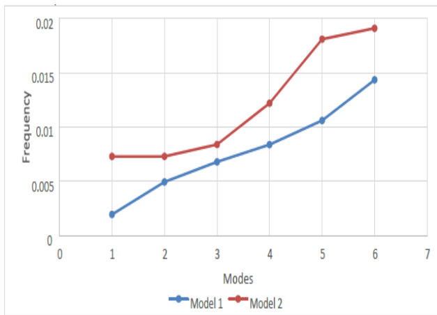
[Graph 7: Frequency Mode for H shape Pylon]
