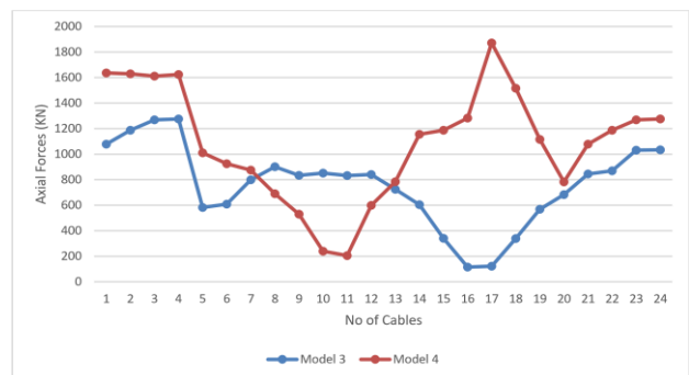
[Graph 2: Comparison between Axial Cable Forces]
