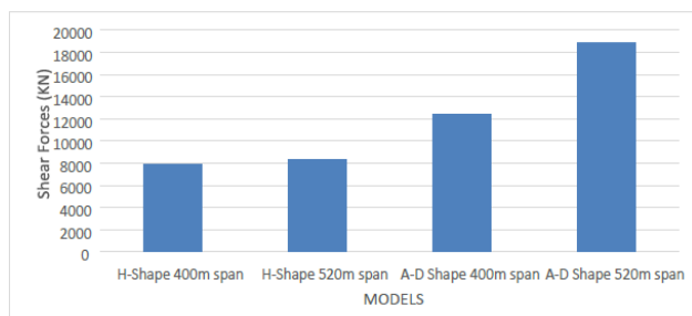
[Graph 10: Variation in Shear Force between H-Type and A-D Type Bridge]
