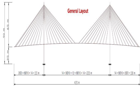
[Fig.1: Bridge Layout]
