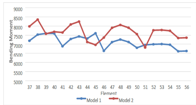
[Graph 5: Variation between Bending Moment]
