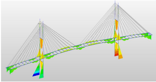
[Fig.4: Bending Moment Post Unknown-Load Factor Optimization]
