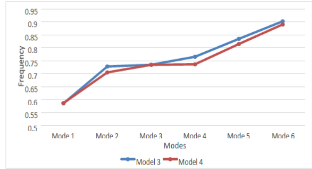
[Graph 8: Frequency Mode for A-D Shape Pylon]
