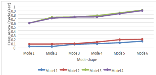
[Graph 12: Variation in Mode Shape Frequency between H-Type and A-D Type Bridge]
