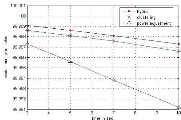
Fig.6 Residual energy of existing and proposed approach
