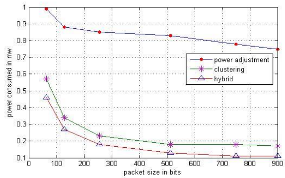
Fig.4 Power consumption at constant data rate(10 kbps)
