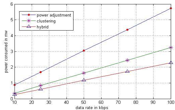
Fig 5 Power consumption at constant packet size(128 bits)
