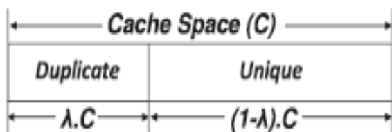
Fig.2. Cache partitioning in split cache policy
