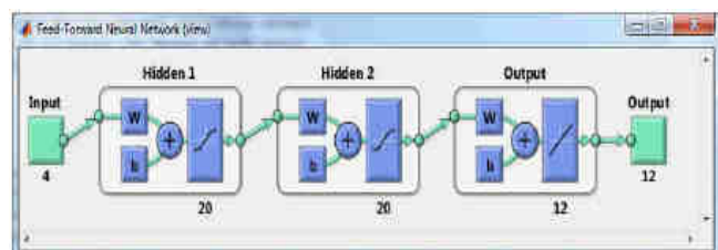
Figure 3.6. Proposed Network Topology
