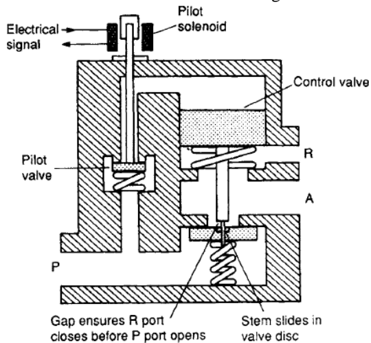
Figure 4.17 Construction of a pilot-operated 3/2 valve Fig 2.1 Solenoid Valve
