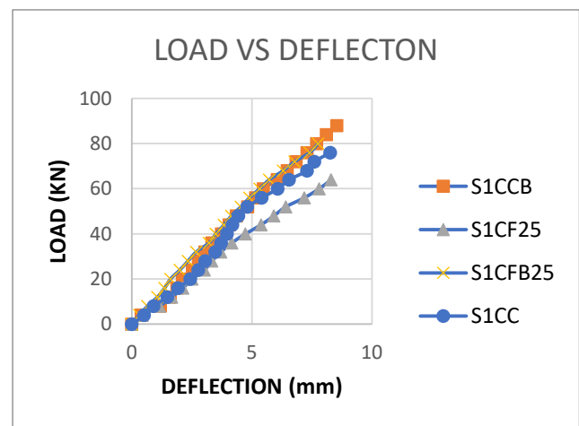
Figure 8 Load vs Deflection on Experimental results
