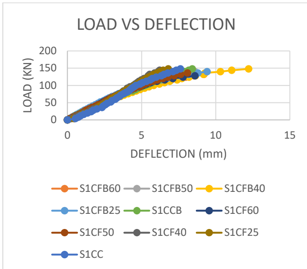
Figure 6 Load vs Deflection on Experimental results
