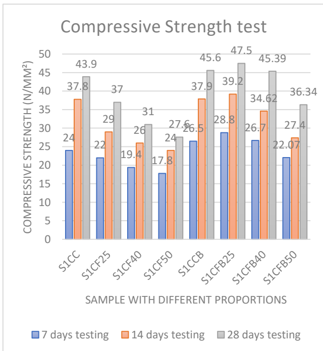
Figure 4 Compressive Strength Test
