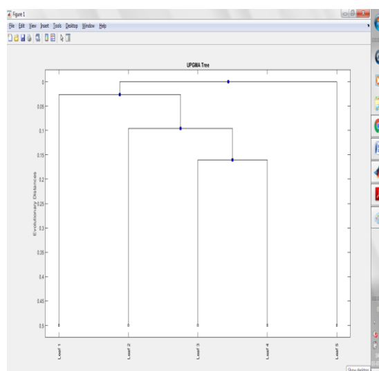
Figure5: UPGMA tree
