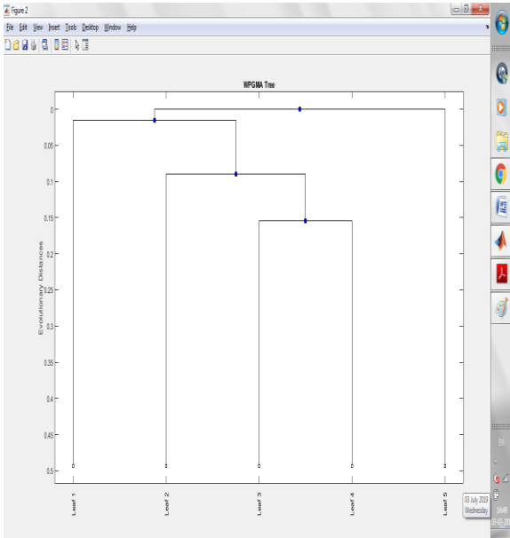
Figure6: WPGMA tree
